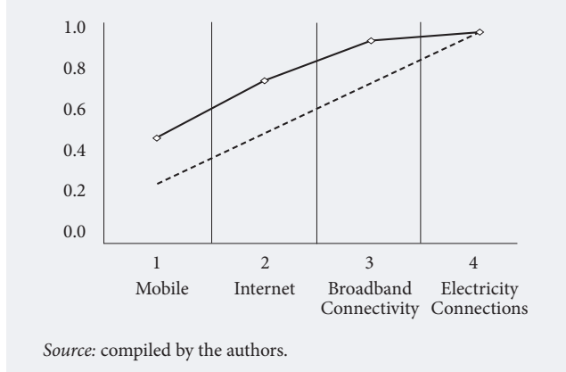
Figure 2. Cumulative Proportions of Eigen Values
